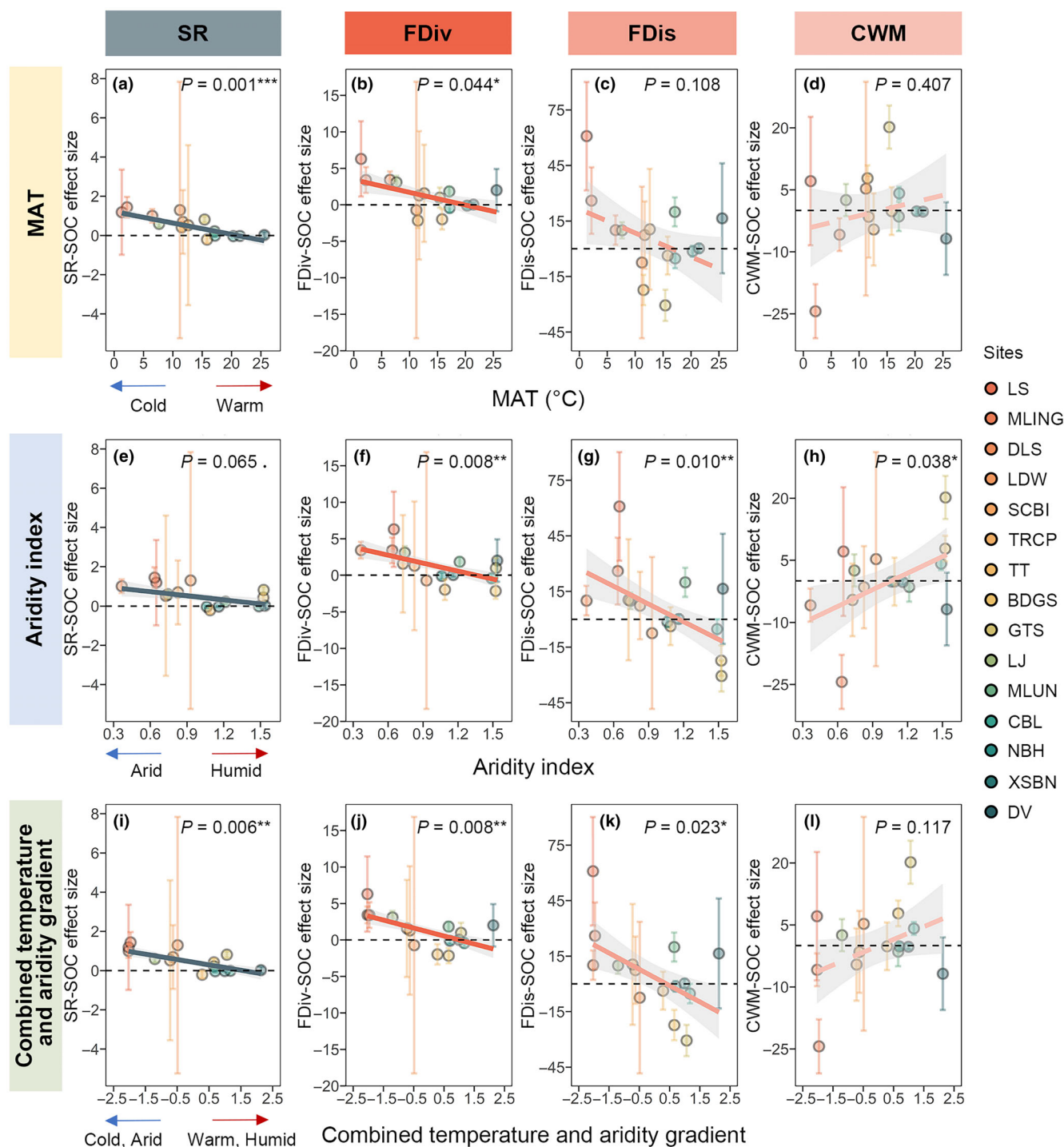
Fig. 4 Relationships between climate and effect sizes of tree diversity–soil organic carbon (SOC) relationships. The relationship between mean annual temperature (MAT) and effect size of SR-SOC (a), FDiv-SOC (b), FDis-SOC (c), and CWM-SOC (d). The relationship between aridity index and effect size of SR-SOC (e), FDiv-SOC (f), FDis-SOC (g), and CWM-SOC (h). The relationship between combined temperature and aridity gradient and effect size of SR-SOC (i), FDiv-SOC (j), FDis-SOC (k), and CWM-SOC (l). Lower values on the x-axes indicate colder, more arid conditions, or both colder and more arid conditions (Combined temperature and aridity gradient). Solid lines show significant ( P < 0.05 ) relationships and dashed lines show nonsignificant ( P > 0.05 ) relationships. ^{***} , P < 0.001 ; ^{**} , P < 0.01 ; ^* , P < 0.05 . The statistical significances were estimated from meta-regression with MAT, Aridity index or combined temperature and aridity gradient as fixed and site as random term. The black dashed line is y = 0 . All tests can be found in Supporting Information Table S10. CWM, community-weighted mean; FDis, functional dispersion; FDiv, functional diversity; SOC, soil organic carbon; SR, species richness.
